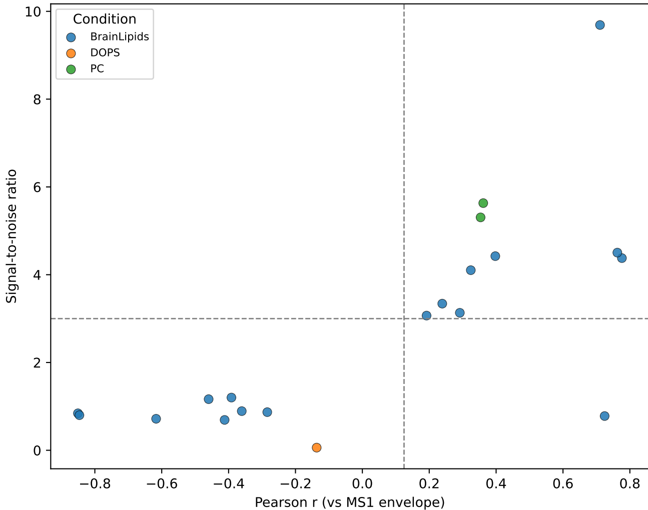
AmtB — Pearson r vs SNR (confident binder = r > 0.125 AND \text{SNR} > 3.0 )
